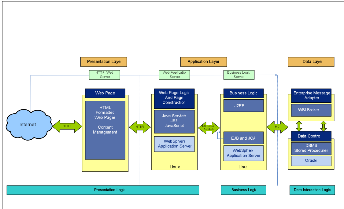
High Level MQ Architecture
